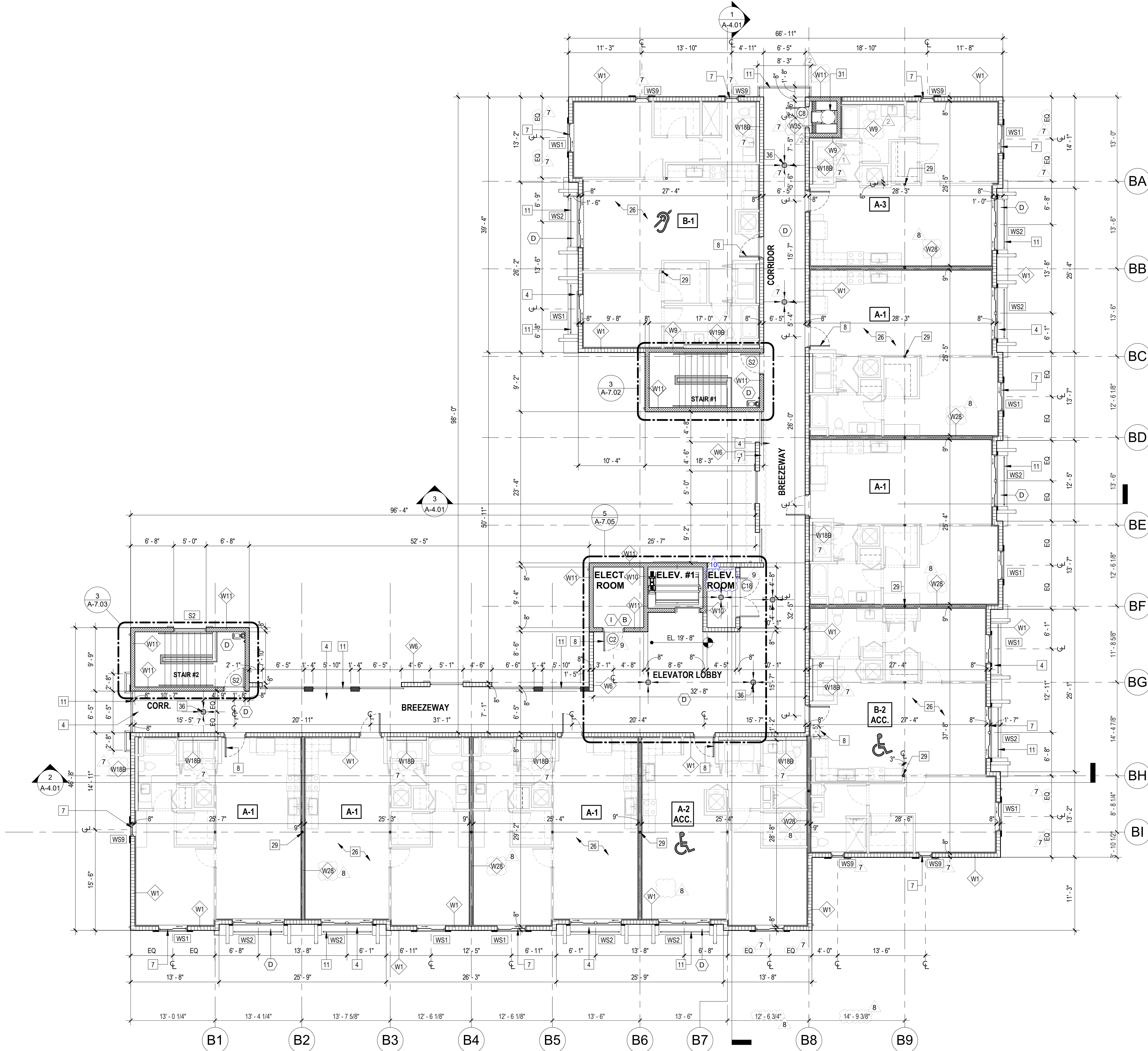
BLDG B - 3RD FLOOR SCALE: 1/8" = 1'-0"
